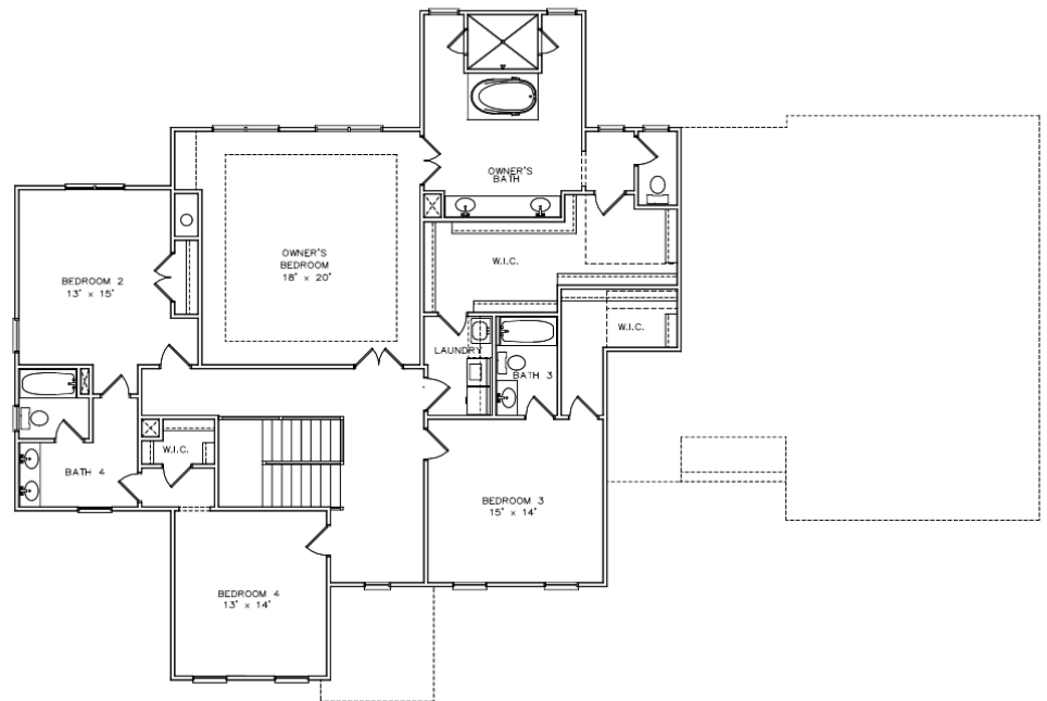
Second Floor
