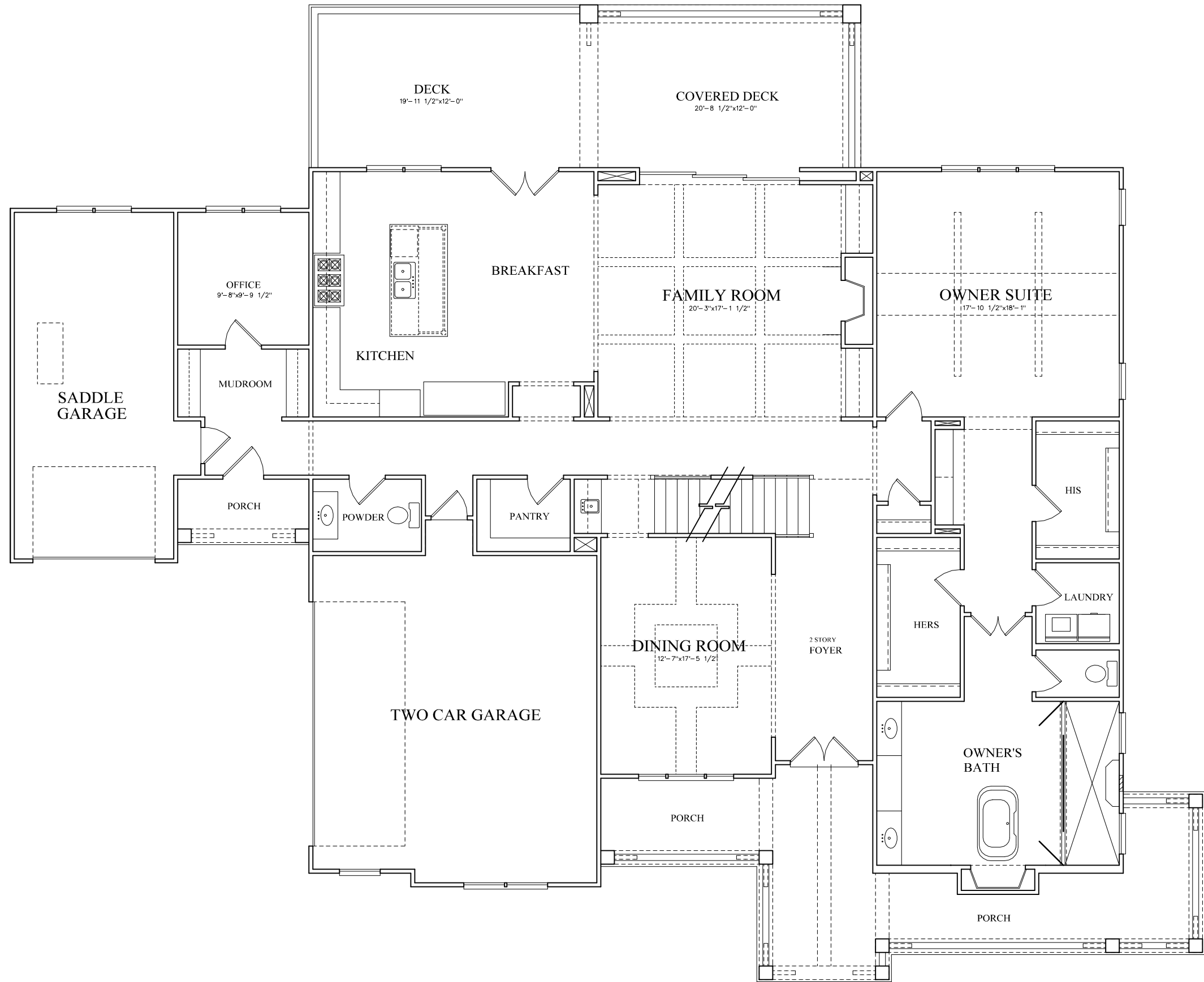
FIRST FLOOR PLAN 2655 Approximate Square Footage
