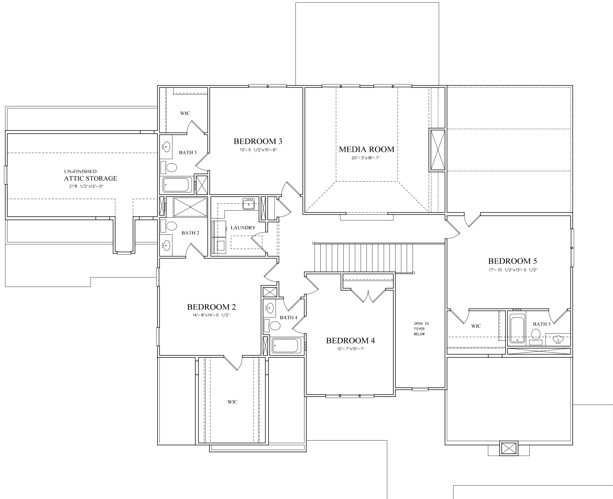
SECOND FLOOR PLAN 2071 Approximate Square Footage
